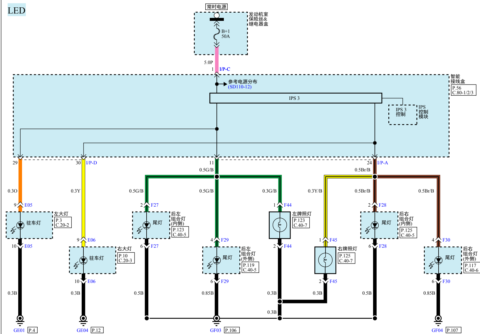
尾灯、驻车灯&amp;牌照灯(3)
